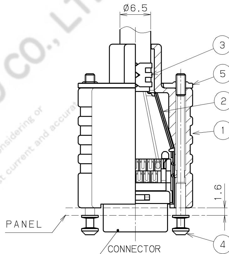
HDR-E26FSG1+ AFTER ASSEMBLY DRAWING
